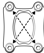
Tighten bolts in an “X” pattern
