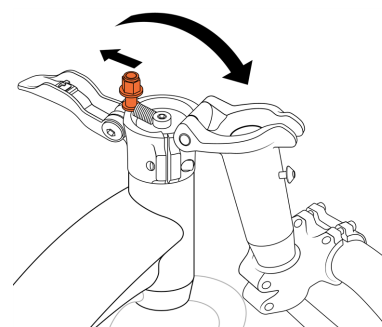
The latch bolt moving forward to allow the stem riser to fold
