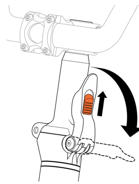
Release the latch on the stem riser.
