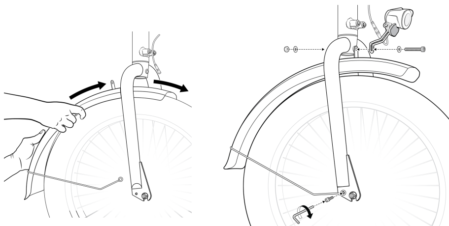
Pass the fender from the back of the front wheel
